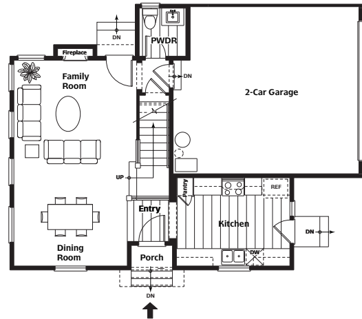
Snowberry (1189-0 A) Main Floor Plan
