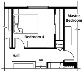
Optional Bedroom 4 Upper Floor Plan
