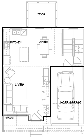
Brackett Main Floor Plan
