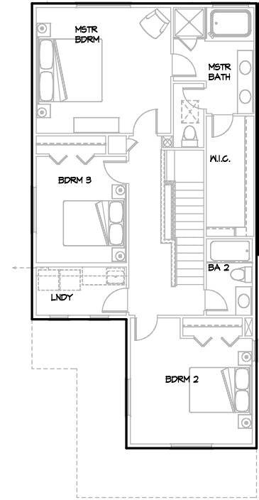
Marymoor Upper Floor Plan
