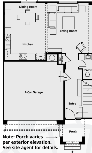
Bridgeport II (1185-5) Main Floor Plan
